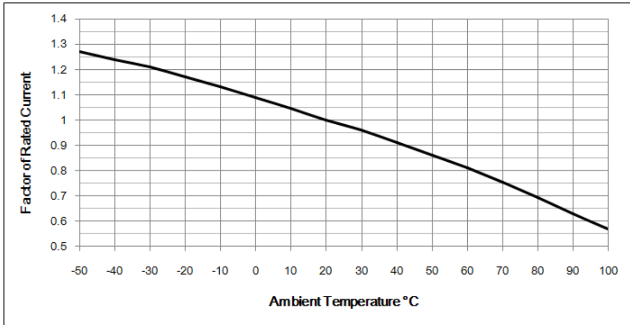
Temperature Re-Rating Curve 温度调(降)额曲线
