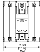
Three Pole
