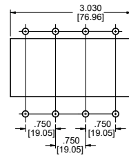
Mounting Detail*
