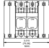
Four Pole
