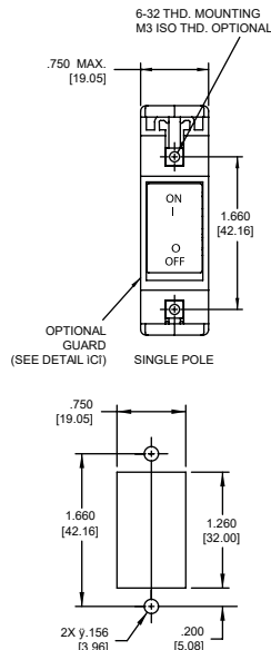
Panel Mounting Detail Mounting Detail Tolerance: \pm .005 [.13] unless noted
