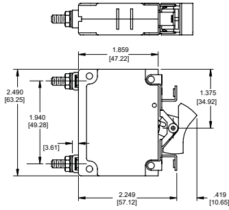
Panel Mounting Detail* Single, Two & Three Pole
