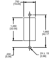
Panel Mounting Detail* Single, Two & Three Pole
